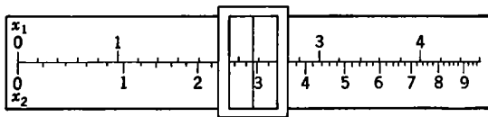
FIG. 3-5.—Nonlinear mechanization of a function of one independent variable.
