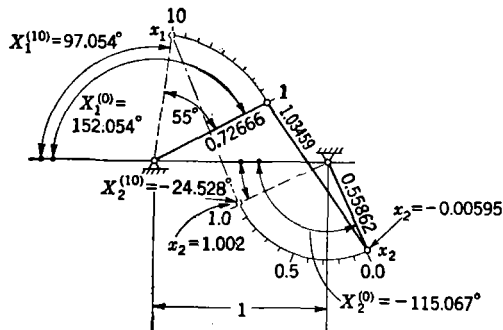
FIG. 7-6.—Second improved logarithmic linkage.
