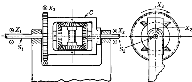
FIG. 1-1.—Bevel-gear differential.
